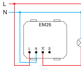
(2) trojičodíkové zapojenie three-wire connection
